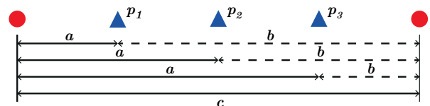
Figure 1: 1-dimensional domain
