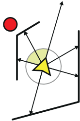
Figure 3: Agent vision
